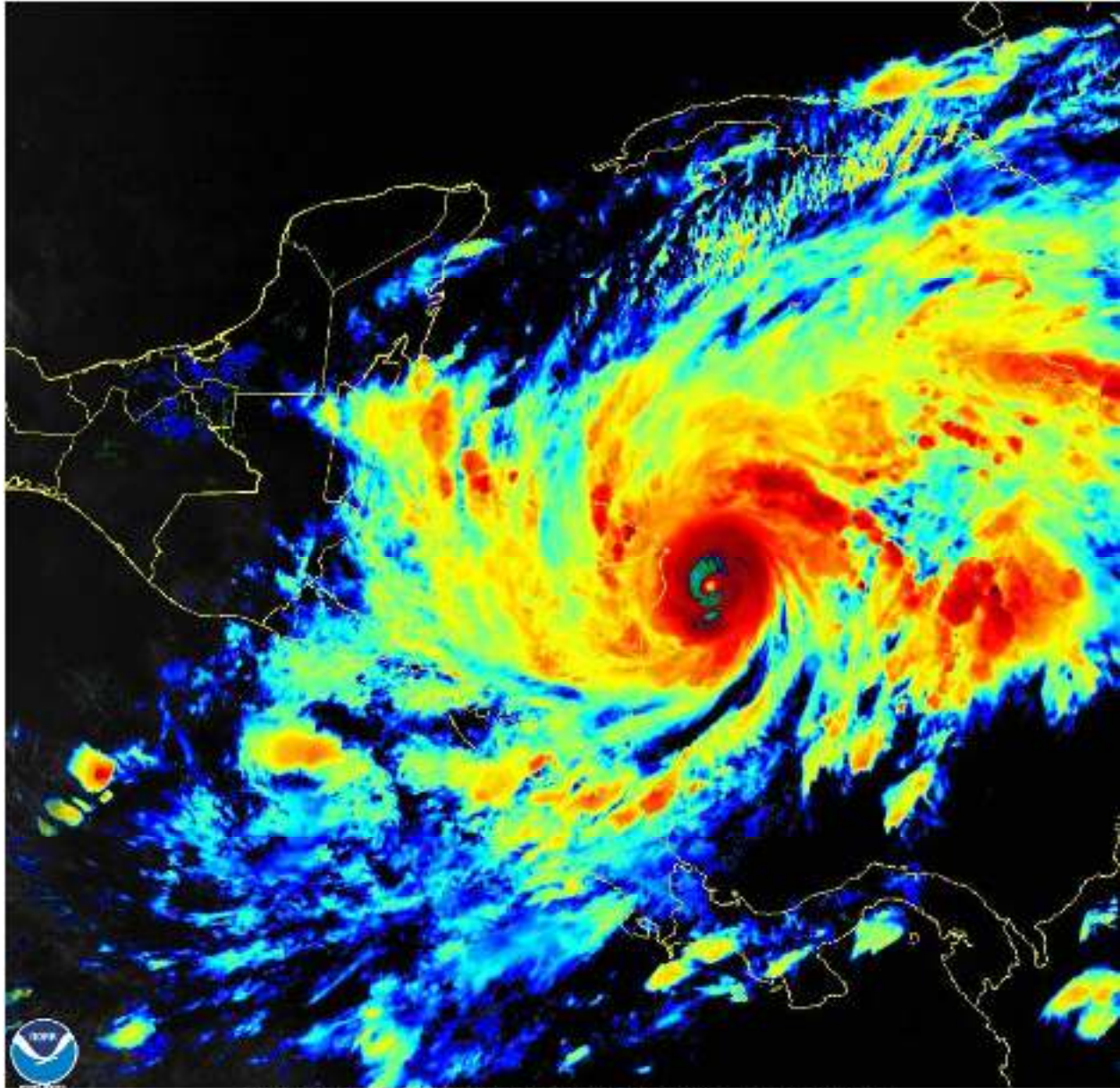
02 Nov 2020 23:40Z NOAA/NESDIS/STAR GOES-East Sandwich
